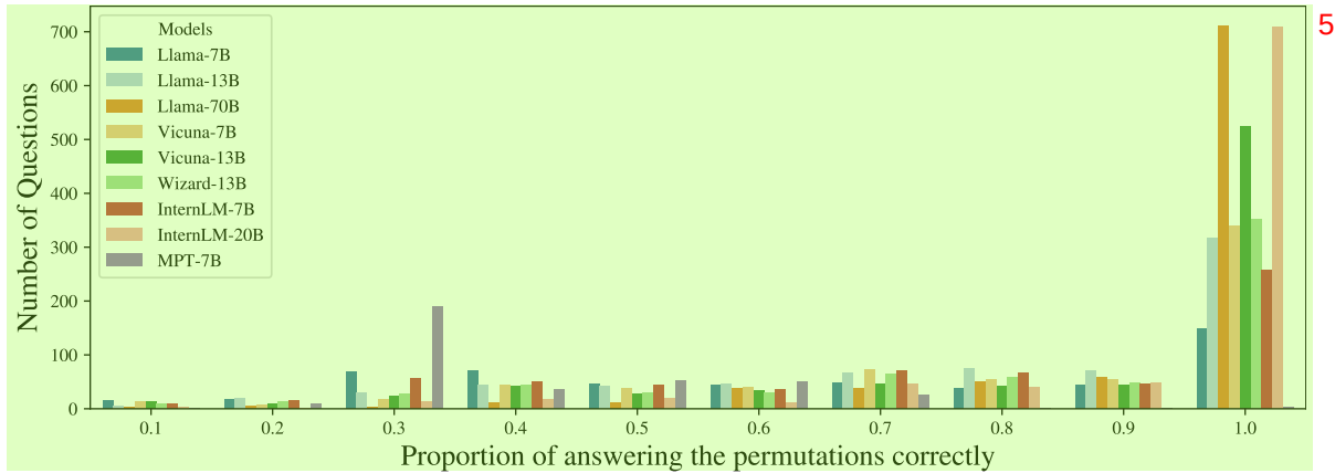
Figure 4. Analysis on permutation distribution. The histogram shows the number of questions for which the corresponding proportion of permutations leads to the correct answer (ideal is a full bar at the 100% bin, indicating that all permutations are correctly answered for all questions). The distribution of bins suggests that many questions have multiple adversarial permutations. 6
