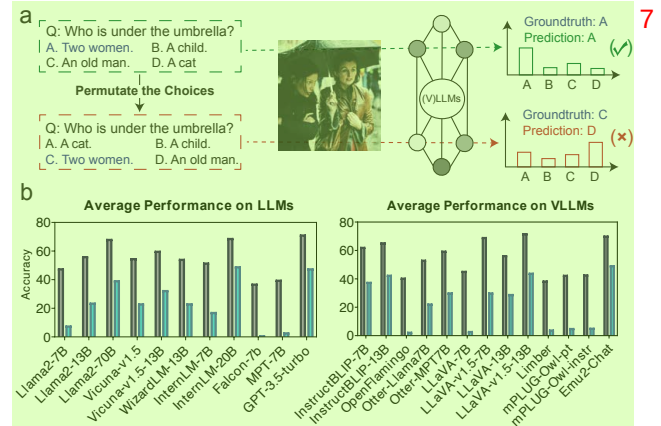
Figure 1. a. Schematic Illustration of an MCQA permutation attack. b. Summary of MCQA adversarial attack results for both LLMs and VLLMs. The values are average accuracy across all benchmarking datasets.
