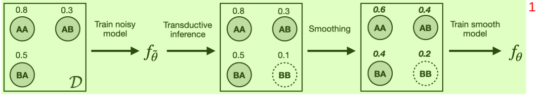
Figure 2: Steps in graph-based smoothing on proteins illustrated with a fictitious data of length 2 sequences with vocabulary \{A, B\} . Above each node are corresponding fitness values. Solid nodes are those in our training set while dashed nodes are augmented via point mutations to increase the smoothing effectiveness. See section 3.2 for description of each step.
