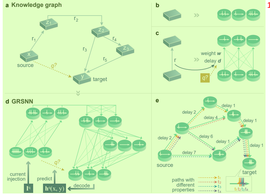
Figure 2. Schematic of GRSNN. (a) Illustration of the graph link prediction task. In GRSNN, (b) each graph entity node is associated with a cluster of spiking neurons, and (c) each relational edge corresponds to the synaptic connections between spiking neurons, with synaptic weight and delay. The weight can exhibit positive or negative values. The delay is contingent on the edge relation and query relation, representing the edge’s property and the neuromodulation from the task goal. (d) Visualization of GRSNN. To predict a link, a constant current, dependent on the query relation, is injected into the spiking neurons of the source node, initiating the propagation of spike trains. After a specific time interval, the spike trains emanating from the target node are decoded to predict the query relation. (e) Depiction of the temporal domain serving as an additional dimension to process the properties of edges and paths in a network with more propagation paths. In the demonstrated network under a simplified setting where each input spike triggers an output spike for neurons, a spike from the source neuron will lead to four spikes from the target neuron, whose time varies corresponding to four propagation paths with different integrated properties of edges represented by synaptic delay.
