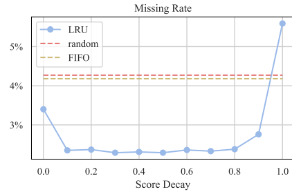
Figure 4: Missing rates of different cache management strategies.
