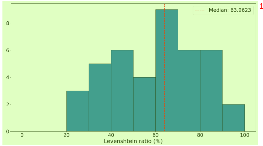
Figure D. Levenshtein ratio between autoformalized and repaired Elements proofs generated by GPT-4V (5-shot).
