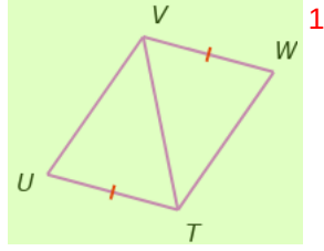
Figure B. Diagrammatic input for UniGeo proof/Congruent Thm02
