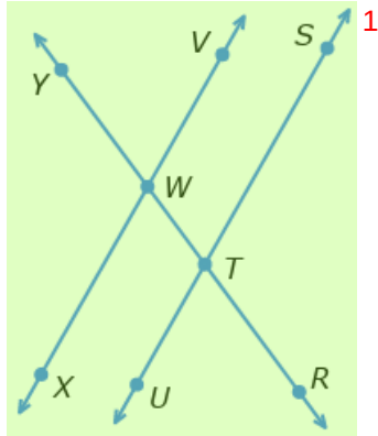
Figure F. Diagrammatic input for UniGeo/Parallel/Thm06 2
