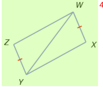
Figure E. Diagrammatic input for UniGeo/Congruent/Thm07 5
