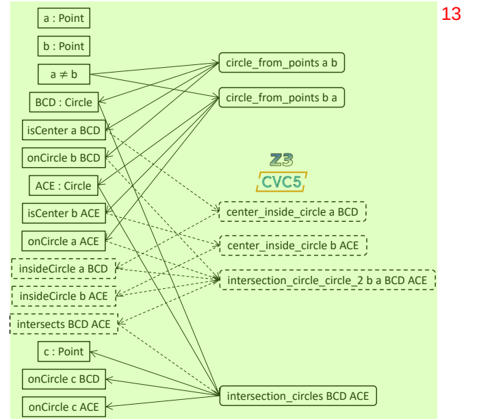
Figure 2. Three steps in the proof in Fig. 1. Left: Geometric 14 objects and facts. Right: Rules applied to construct new objects and deduce new facts. Each rule has inbound arrows from its preconditions and outbound arrows to its postconditions. Dashed lines: When applying a rule with missing preconditions, we try to fill the gap using a symbolic reasoning engine based on SMT solvers. These implicit steps performed by the symbolic engine can only use non-construction rules, whereas explicit steps performed by humans (or machine learning models) can use any rules.
