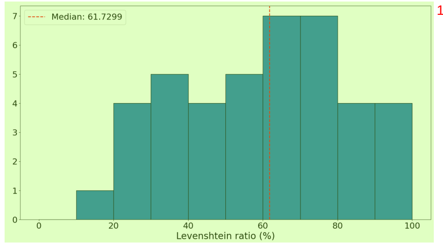
Figure C. Levenshtein ratio between autoformalized and repaired Elements proofs generated by GPT-4 (5-shot).
