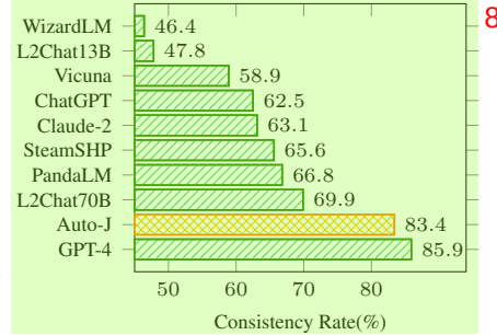
Figure 4: Consistency of prediction when swapping the response order.
