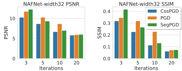
Figure 8: Non-targeted \ell_\infty -norm constrained CosPGD, PGD, and SegPGD attacks on NAFNet, recently proposed by (Chen et al., 2022) as the state-of-the-art network for image de-blurring on the GoPro dataset. CosPGD significantly outperforms the other attacks. Lower PSNR and SSIM indicate a worse restoration and thus a stronger attack.
