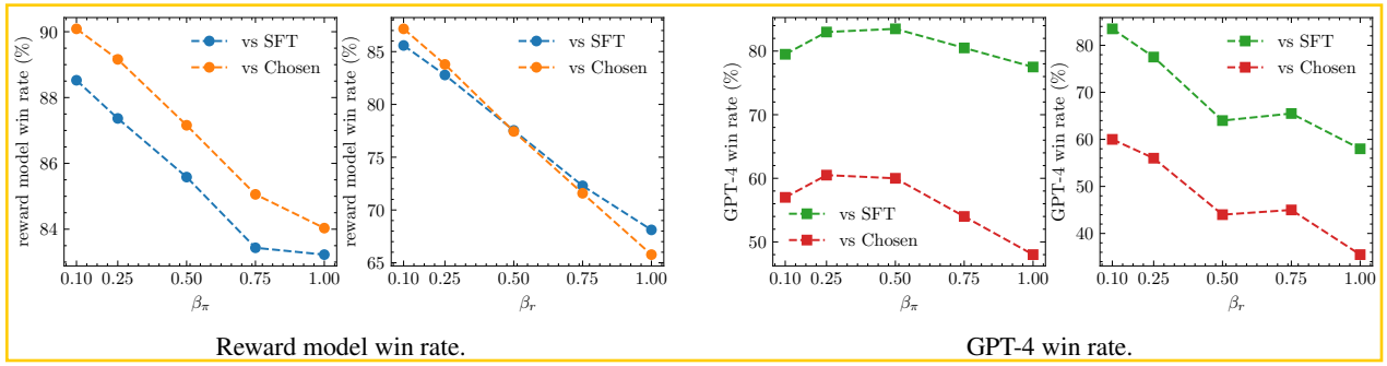
Figure 6. Win rate performance of \text{EXO}_{\text{rw}} evaluated by the reward model and the GPT-4 by varying \beta_r and \beta_\pi .
