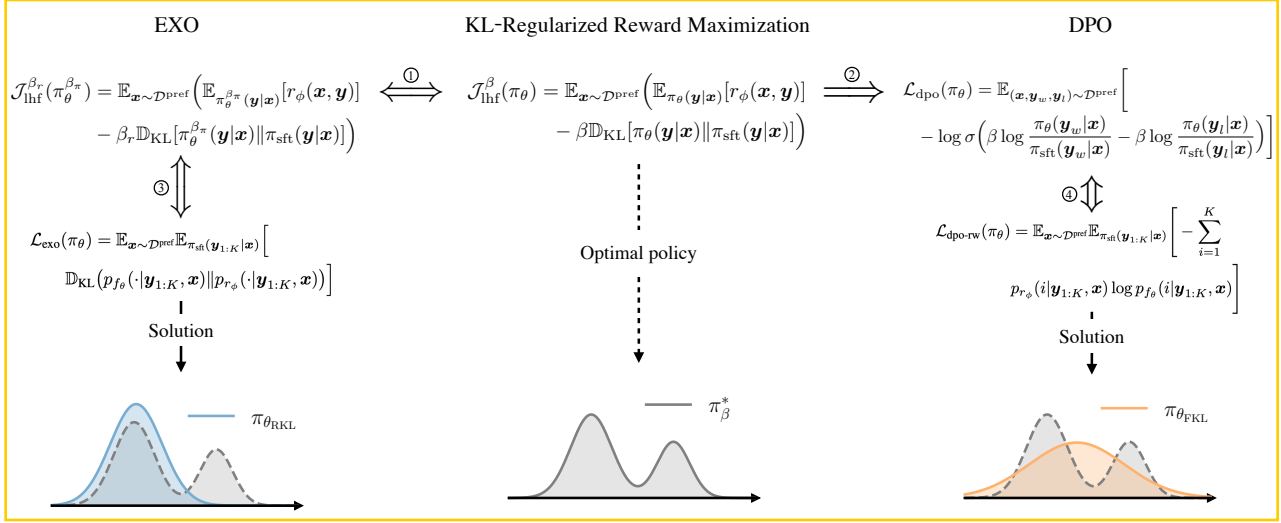
Figure 5. Illustration of the relationship among the different objectives discussed in §3. (1) \mathcal{J}_{\text{hlf}}^{\beta_r}(\pi_\theta^{\beta_\pi}) is a generalized version of \mathcal{J}_{\text{hlf}}^\beta(\pi_\theta) by distributing the KL regularization to both the learned policy \pi_\theta and the reward model r_\phi (§3.1). (2) \mathcal{L}_{\text{dpo}}(\pi_\theta) is derived based on the optimal policy of \mathcal{J}_{\text{hlf}}^\beta(\pi_\theta) (§2.3). (3) \mathcal{L}_{\text{exo}}(\pi_\theta) is equivalent to \mathcal{J}_{\text{hlf}}^{\beta_r}(\pi_\theta^{\beta_\pi}) in terms of their optimization directions (§3.2). (4) \mathcal{L}_{\text{dpo-rw}} is the generalized version of \mathcal{L}_{\text{dpo}} by substituting the pairwise loss with softmax loss over K responses (§3.3). The optimal policy, denoted by a dotted line, assumes unlimited model capacity. The solution, shown with a solid line, is the practically achievable policy within the realistic constraints of model capacity.
