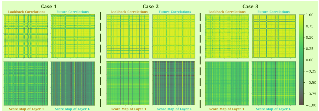
Figure 11: Multivariate correlations of the lookback series and future series and the learned score 9 maps by inverted self-attention of different layers. Cases all come from the Solar-Energy dataset.
