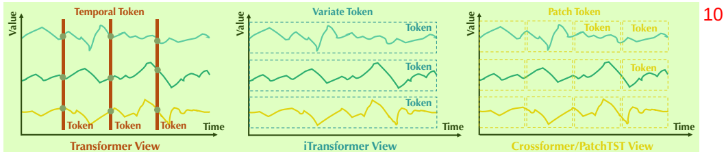
Figure 19: Tokenizations for multivariate time series modality of representative Transformers. 11
