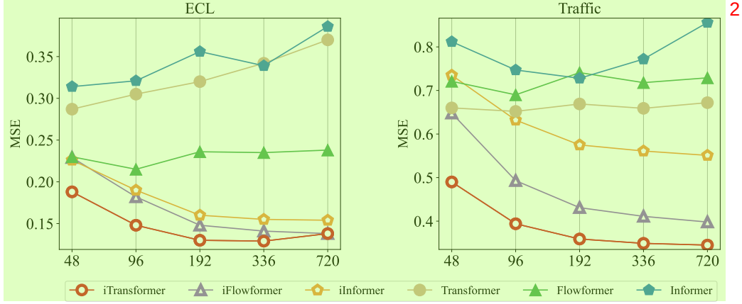
Figure 6: Forecasting performance with the lookback length T \in \{48, 96, 192, 336, 720\} and fixed prediction length S = 96 . While the performance of Transformer-based forecasters does not necessarily benefit from the increased lookback length, the inverted framework empowers the vanilla Transformer and its variants with improved performance on the enlarged lookback window.
