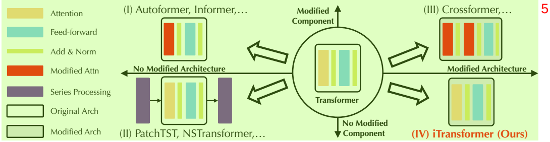
Figure 3: Transformer-based forecasters categorized by component and architecture modifications. 6
