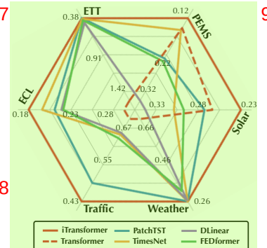
Figure 1: Performance of iTransformer. Average results (MSE) are reported following TimesNet (2023).
