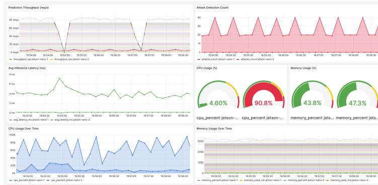
Figure 3. Grafana dashboard at peak load in the split deployment: the anomaly-gate node (jetson-nano-1) uses about 5% CPU while the PySpark classifier node (jetson-nano-2) reaches roughly 91%, showing the load asymmetry between the two pipeline roles.
