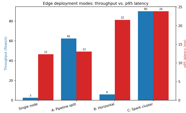
Figure 7. Throughput and p95 latency across deployment modes.
