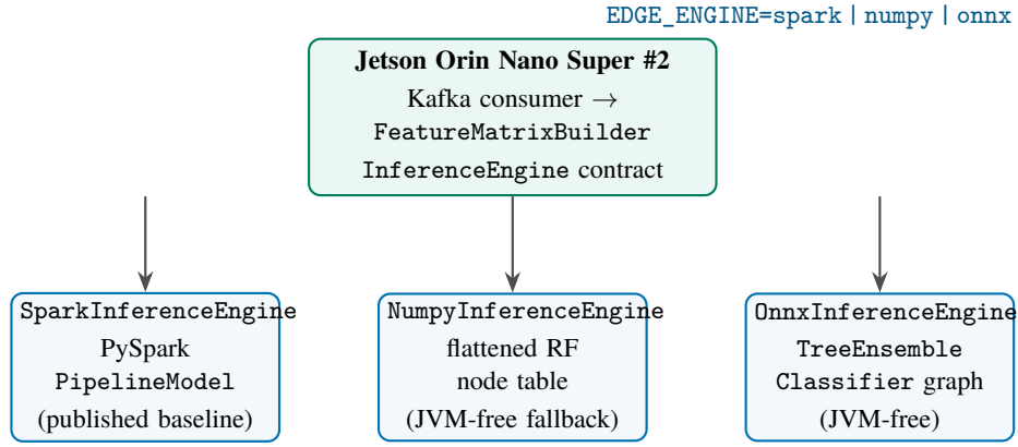
Fig. 1. Swappable classifier tier on Jetson #2: one feature-matrix builder, one InferenceEngine contract, three backends selected by a single environment variable. The gate on Jetson #1 and the Kafka/monitoring topology are unchanged from the companion paper.
