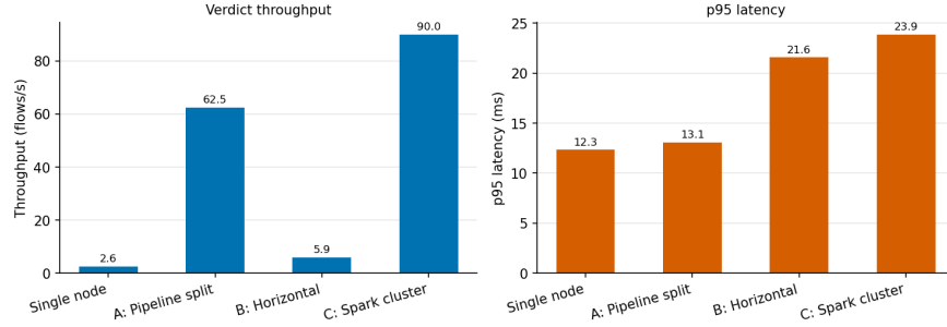
Fig. 6. Deployment-mode comparison: verdict throughput (left) and p95 latency (right).
