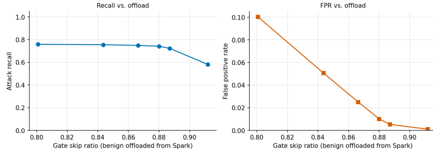
Fig. 7. Anomaly-gate operating curve: attack recall (left) and false-positive rate (right) vs. gate-skip ratio.
