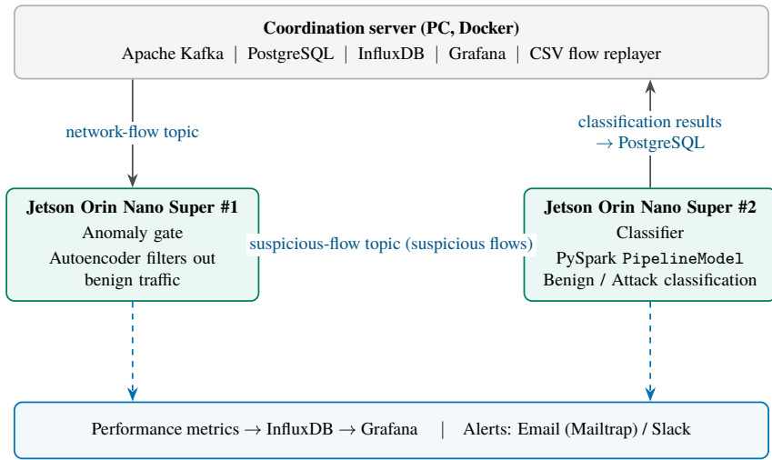
Fig. 1. Split-deployment architecture (PC + 2 × Jetson Orin Nano Super).
