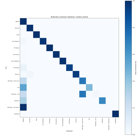
Figure 4. Multiclass confusion matrix (row-normalized).
