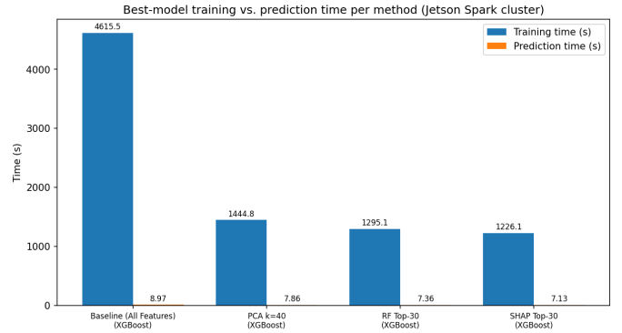
Figure 4. Training and inference time of the representative model of each method, measured on the Spark cluster used for training (Section IV); inference latency/throughput measurements on the edge device belong to a companion systems paper (under submission), not this paper.
