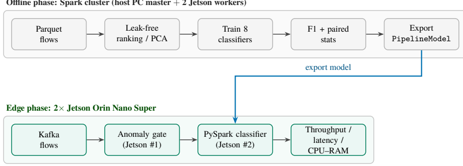
Fig. 5. Two-phase train-deploy pipeline linking Spark ML experiments to Jetson edge inference.
