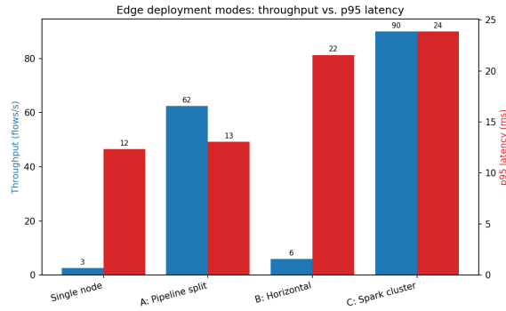
Figure 7. Throughput and p95 latency across deployment modes.
