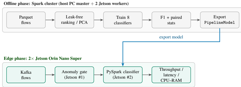
Figure 5. Two-phase train-deploy pipeline linking Spark ML experiments to Jetson edge inference.
