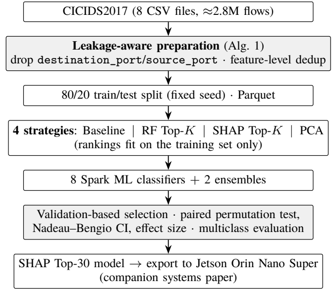
Figure 1. Leakage-aware evaluation pipeline: from raw CICIDS2017 flows to the statistically validated, edge-ready model.
