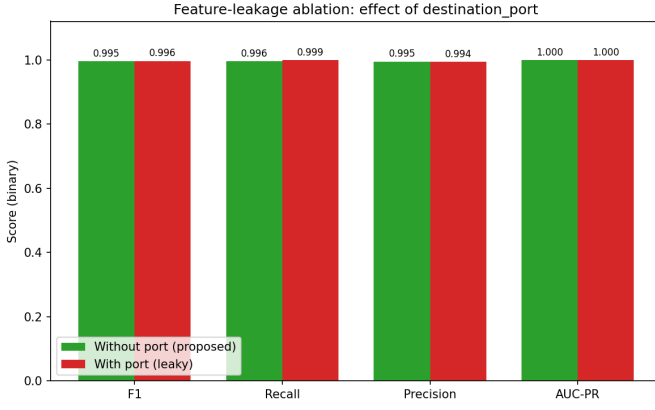
Figure 2. Impact of the leaking feature destination_port (Random Forest, binary).
