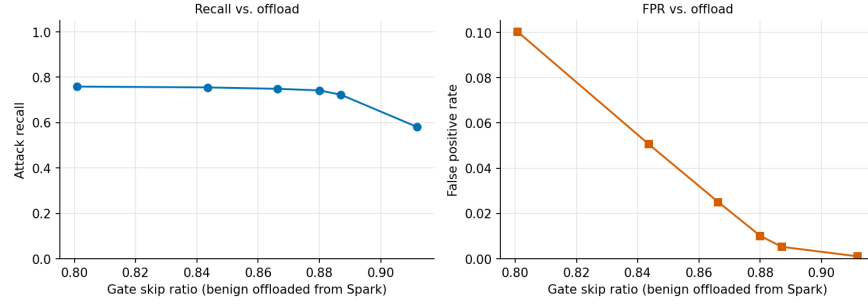
Figure 8. Anomaly-gate operating curve: attack recall (left) and false-positive rate (right) vs. gate-skip ratio.
