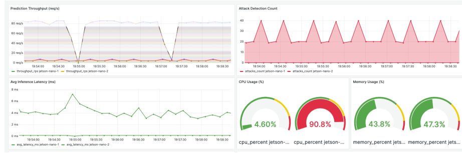
Fig. 3. Grafana dashboard at peak load in the split deployment: the anomaly-gate node ( jetson-nano-1 ) uses 4.6% CPU while the PySpark classifier node ( jetson-nano-2 ) reaches 90.8%, showing the load asymmetry between the two pipeline roles.
