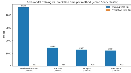
Figure 3. Training and inference time of each method’s representative model on the training Spark cluster (Section IV).
