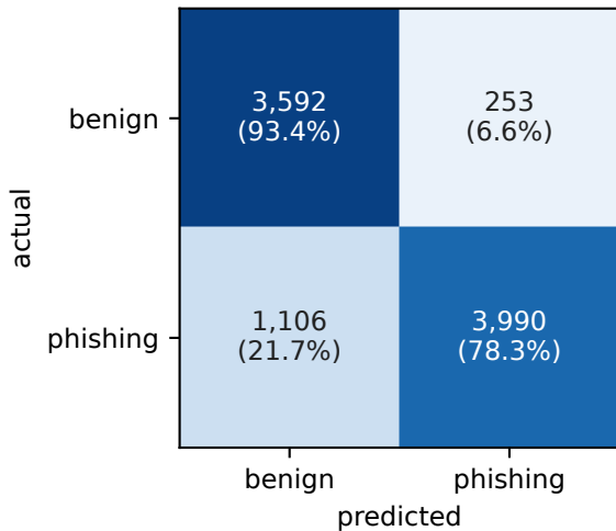
HistGB (21 features)
