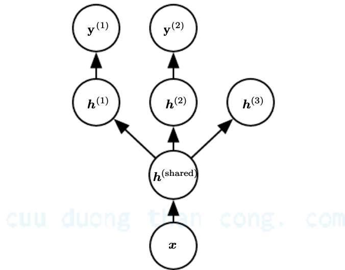
Figure 7.2: Multi-task learning can be cast in several ways in deep learning frameworks and this figure illustrates the common situation where the tasks share a common input but involve different target random variables. The lower layers of a deep network (whether it is supervised and feedforward or includes a generative component with downward arrows) can be shared across such tasks, while task-specific parameters (associated respectively with the weights into and from \mathbf{h}^{(1)} and \mathbf{h}^{(2)} ) can be learned on top of those yielding a shared representation \mathbf{h}^{(\text{shared})} . The underlying assumption is that there exists a common pool of factors that explain the variations in the input \mathbf{x} , while each task is associated with a subset of these factors. In this example, it is additionally assumed that top-level hidden units \mathbf{h}^{(1)} and \mathbf{h}^{(2)} are specialized to each task (respectively predicting \mathbf{y}^{(1)} and \mathbf{y}^{(2)} ) while some intermediate-level representation \mathbf{h}^{(\text{shared})} is shared across all tasks. In the unsupervised learning context, it makes sense for some of the top-level factors to be associated with none of the output tasks ( \mathbf{h}^{(3)} ): these are the factors that explain some of the input variations but are not relevant for predicting \mathbf{y}^{(1)} or \mathbf{y}^{(2)} .
