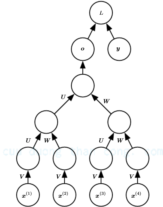
Figure 10.14: A recursive network has a computational graph that generalizes that of the recurrent network from a chain to a tree. A variable-size sequence \mathbf{x}^{(1)}, \mathbf{x}^{(2)}, \dots, \mathbf{x}^{(t)} can be mapped to a fixed-size representation (the output \mathbf{o} ), with a fixed set of parameters (the weight matrices \mathbf{U} , \mathbf{V} , \mathbf{W} ). The figure illustrates a supervised learning case in which some target \mathbf{y} is provided which is associated with the whole sequence.
