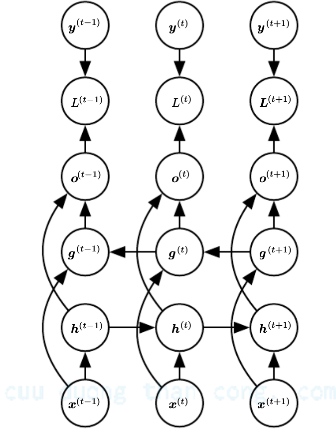
Figure 10.11: Computation of a typical bidirectional recurrent neural network, meant to learn to map input sequences \mathbf{x} to target sequences \mathbf{y} , with loss L^{(t)} at each step t . The \mathbf{h} recurrence propagates information forward in time (towards the right) while the \mathbf{g} recurrence propagates information backward in time (towards the left). Thus at each point t , the output units \mathbf{o}^{(t)} can benefit from a relevant summary of the past in its \mathbf{h}^{(t)} input and from a relevant summary of the future in its \mathbf{g}^{(t)} input.
