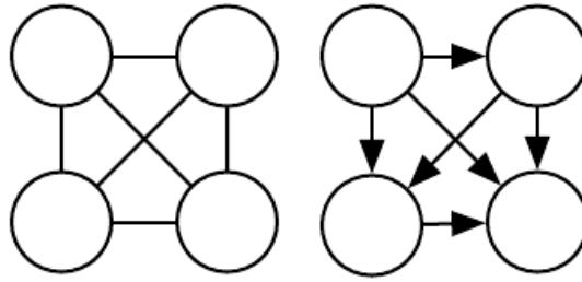
Figure 16.10: Examples of complete graphs, which can describe any probability distribution. Here we show examples with four random variables. ( Left )The complete undirected graph. In the undirected case, the complete graph is unique. ( Right )A complete directed graph. In the directed case, there is not a unique complete graph. We choose an ordering of the variables and draw an arc from each variable to every variable that comes after it in the ordering. There are thus a factorial number of complete graphs for every set of random variables. In this example we order the variables from left to right, top to bottom.
