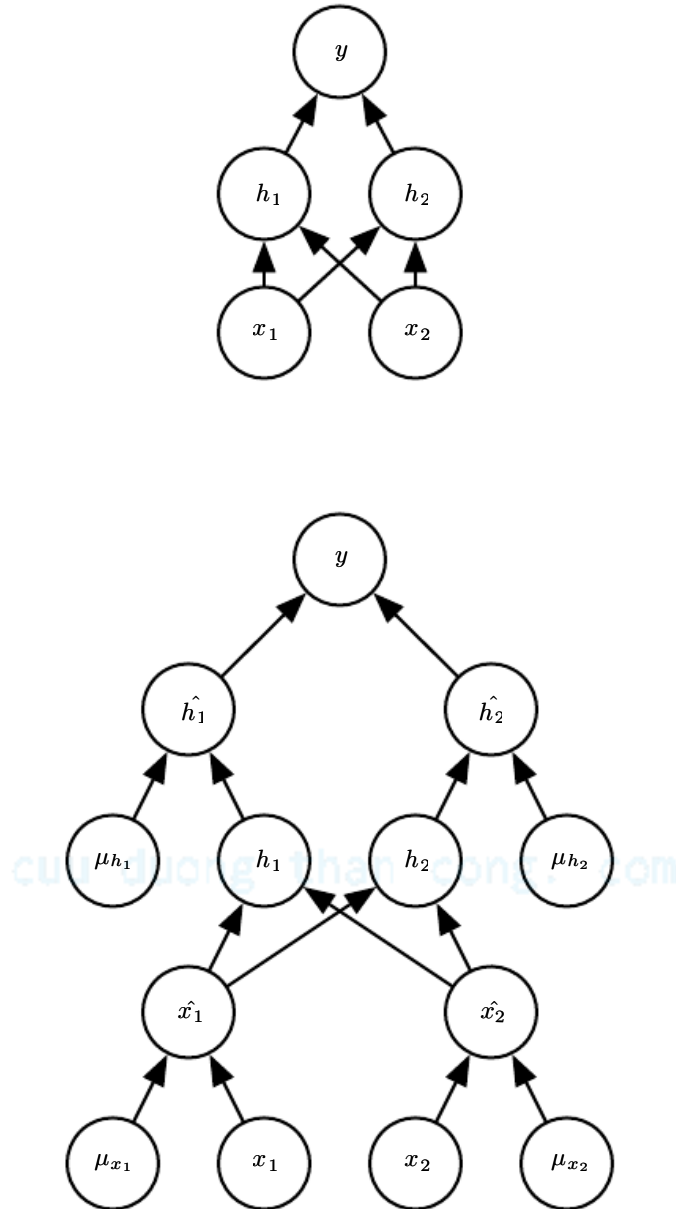
Figure 7.7: An example of forward propagation through a feedforward network using dropout. ( Top ) In this example, we use a feedforward network with two input units, one hidden layer with two hidden units, and one output unit. ( Bottom ) To perform forward propagation with dropout, we randomly sample a vector \boldsymbol{\mu} with one entry for each input or hidden unit in the network. The entries of \boldsymbol{\mu} are binary and are sampled independently from each other. The probability of each entry being 1 is a hyperparameter, usually 0.5 for the hidden layers and 0.8 for the input. Each unit in the network is multiplied by the corresponding mask, and then forward propagation continues through the rest of the network as usual. This is equivalent to randomly selecting one of the sub-networks from figure 7.6 and running forward propagation through it.
