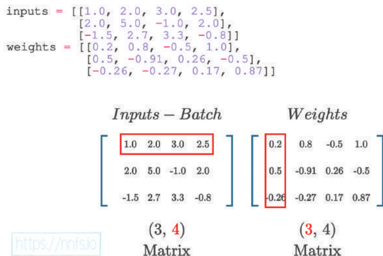
Fig 2.18: Depiction of why we need to transpose to perform the matrix product.
