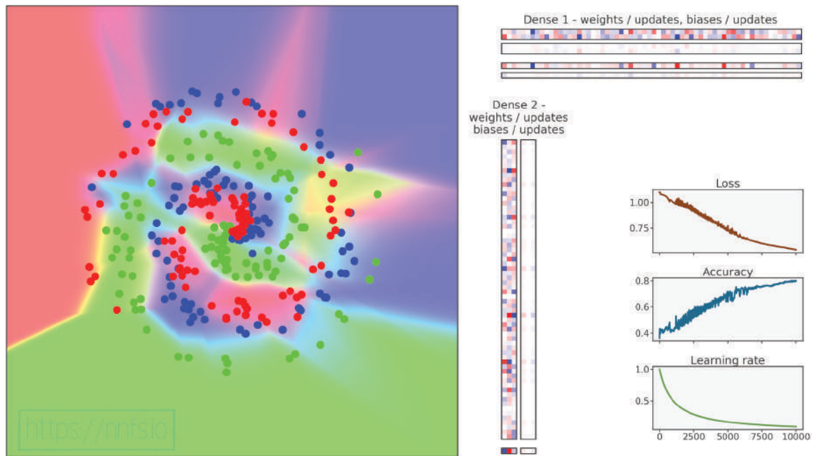
Fig 10.18: Model training with SGD optimizer, learning rate decay and Momentum.
