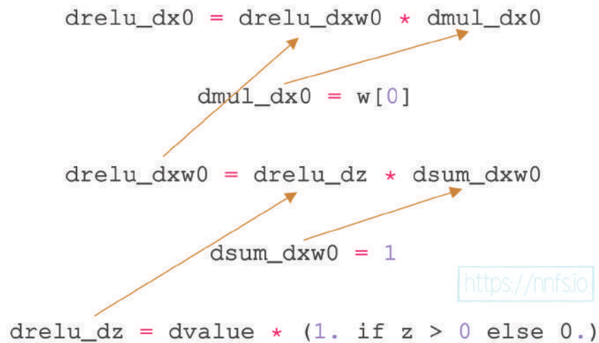
Fig 9.20: How to apply the chain rule for the partial derivative of ReLU w.r.t. first input
