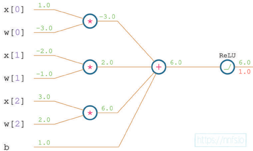
Fig 9.06: Initial gradient (received during backpropagation).
