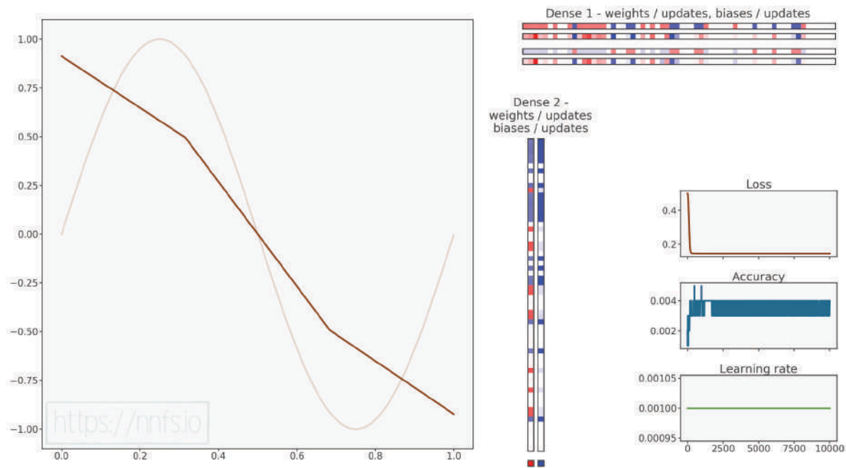
Fig 17.03: Model stopped training immediately.
