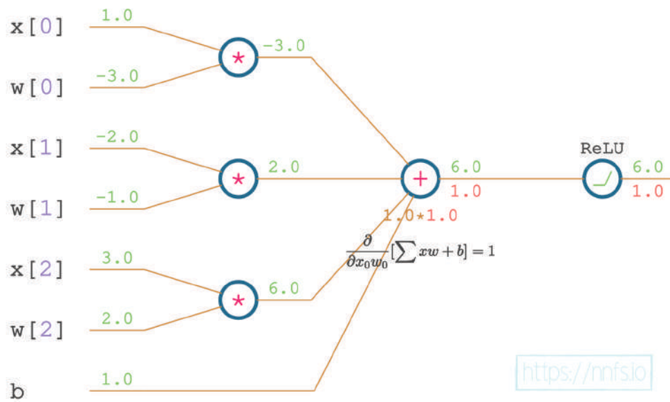
Fig 9.09: Partial derivative of the sum function w.r.t. the first weighted input; the chain rule.
