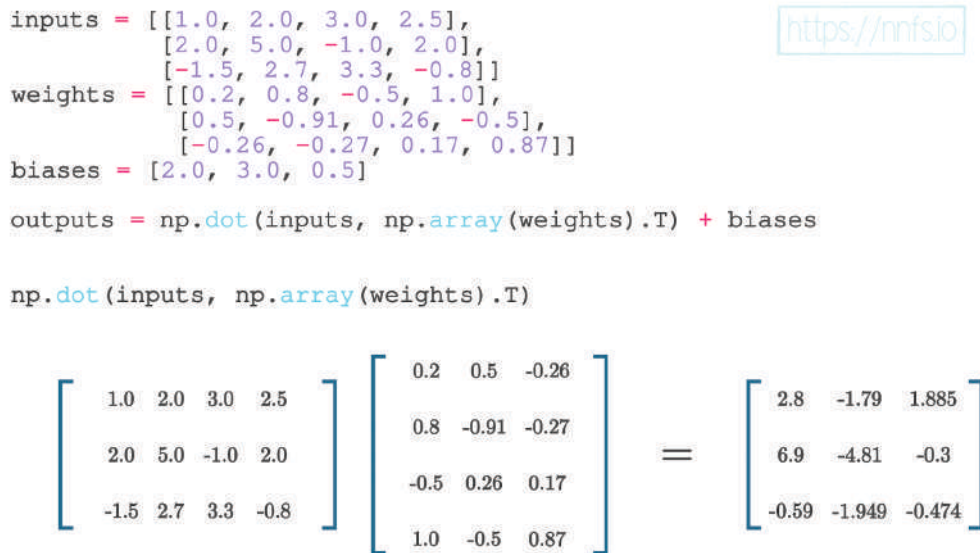
Fig 2.20: Code and visuals depicting the dot product of inputs and transposed weights.
