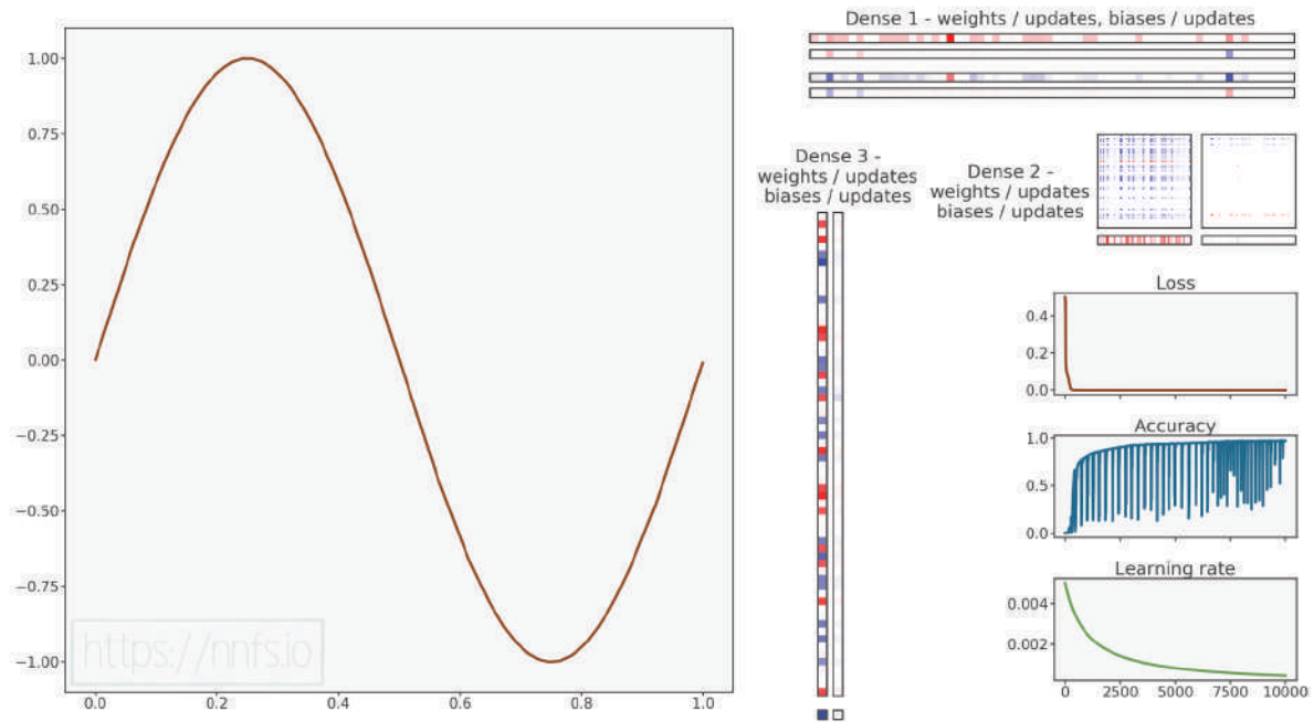
Fig 17.11: Model trained to fit the sine data.
