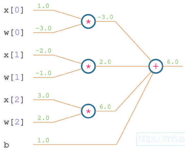
Fig 9.04: Weighted inputs and bias addition.
