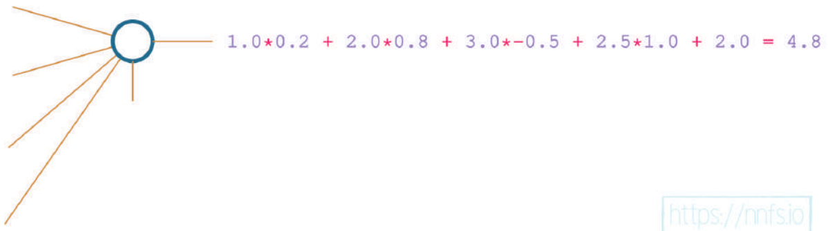
Fig 2.03: Visualizing the code that makes up a basic neuron, with 4 inputs this time.
