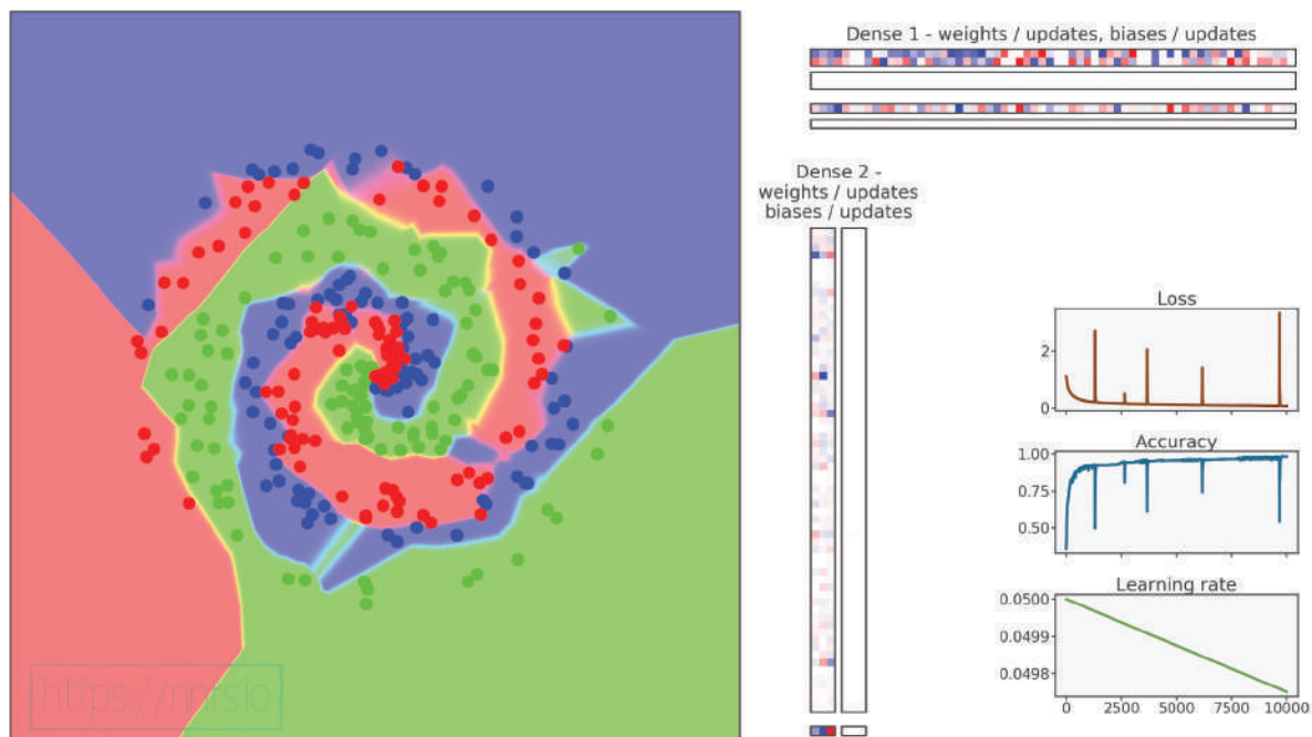
Fig 10.24: Model training with Adam optimizer (tuned).
