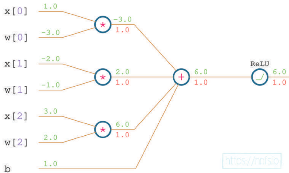
Fig 9.14: The sum and chain rule gradient (for the third weighted input).
