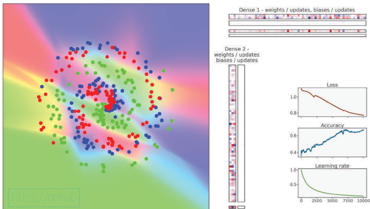
Fig 10.17: Model training with SGD optimizer and more proper learning rate decay.
