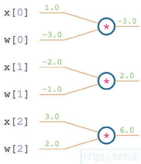
Fig 9.03: Input and weight multiplication of all of the inputs.
