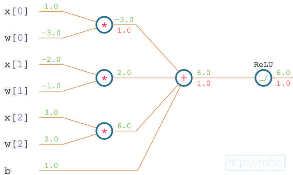
Fig 9.10: The sum and chain rule gradient (for the first weighted input).
