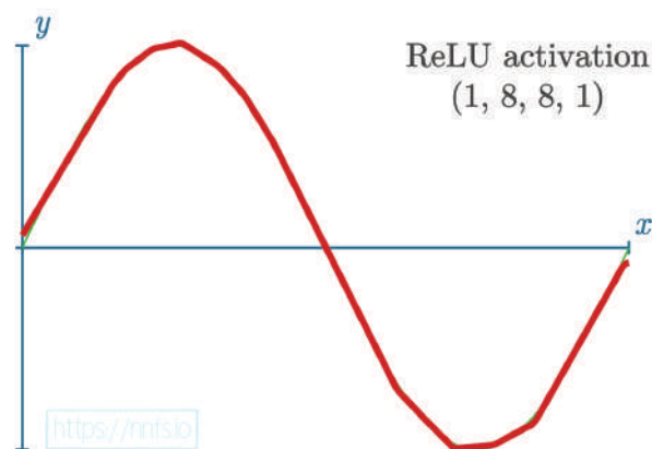
Fig 4.07: ReLU activation functions in hidden layers attempting to fit y=\sin(x)
