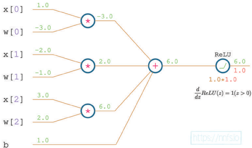
Fig 9.07: Derivative of the ReLU function and chain rule.
