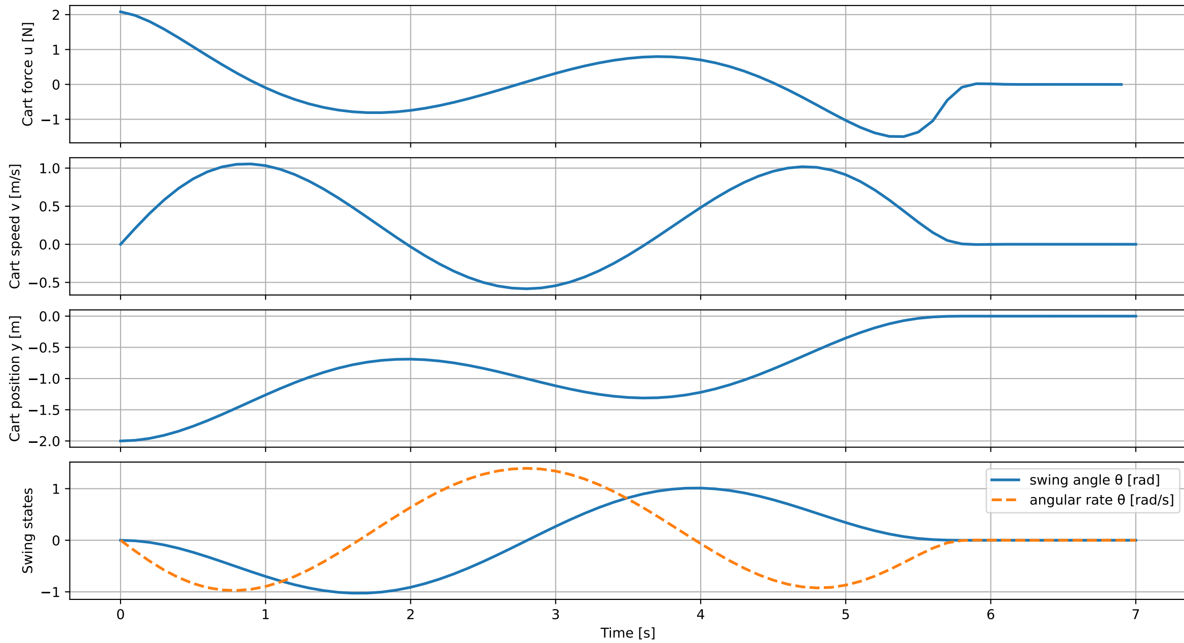
MPC response ( m_2 = 10 kg)
