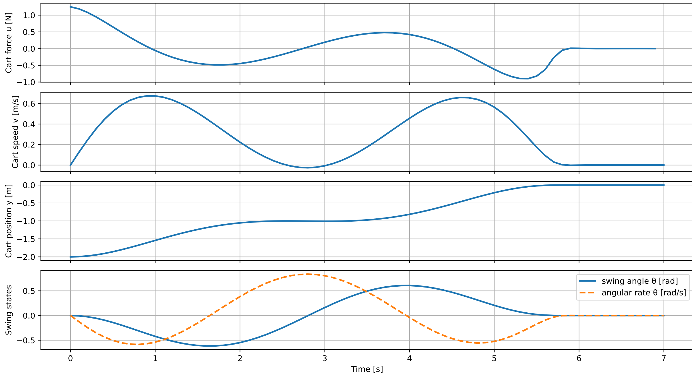
MPC response ( m_2 = 2 kg)
