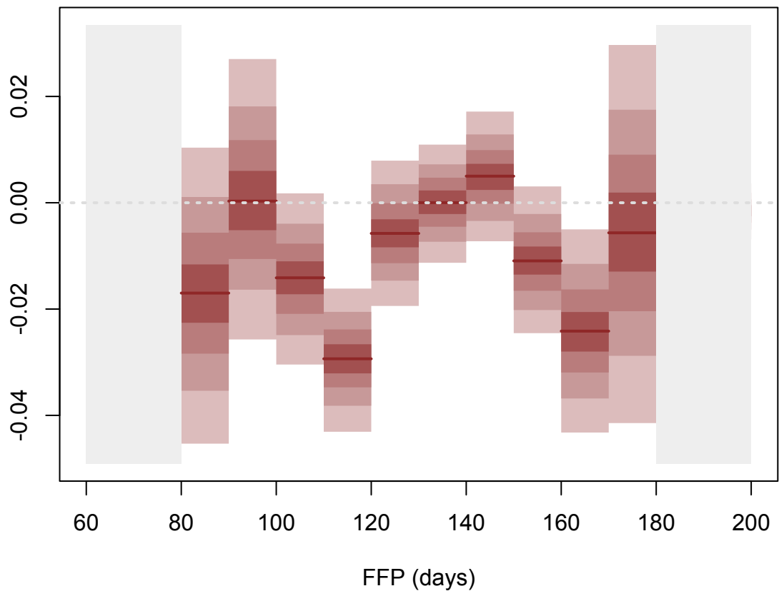
Marginal Quantiles of Conditional Medians - Baselines
