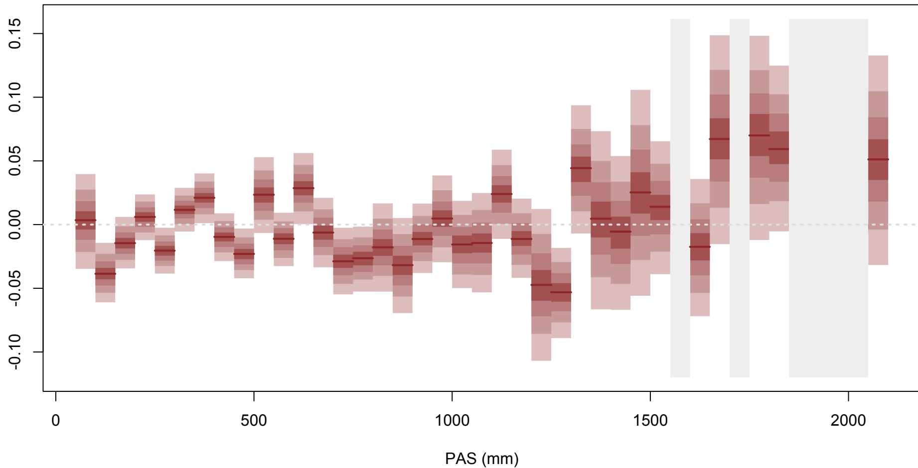
Marginal Quantiles of Conditional Medians - Baselines
