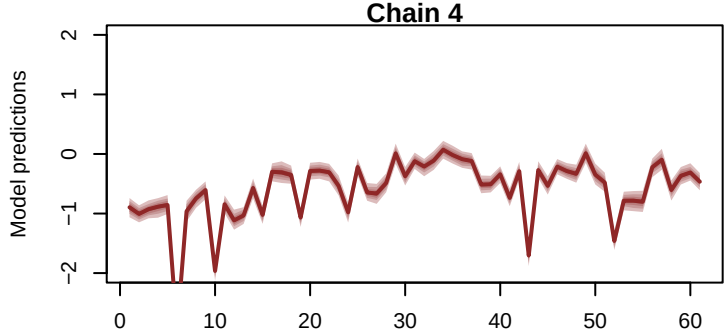
Chain 4
