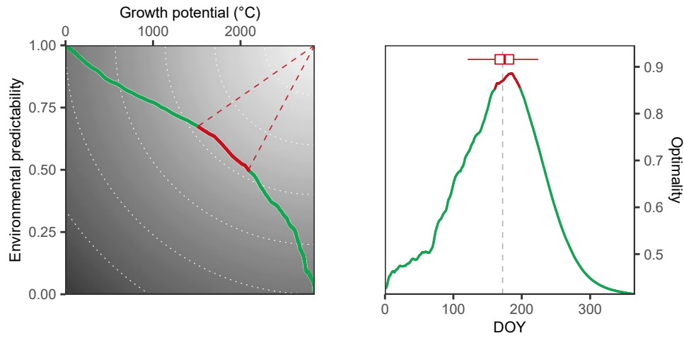
Figure S2: Solstice also marks the average optimal trade-off between environmental predictability and growth potential across North America (1951-2020). The red sections of the green curves represent days where optimality falls within the 90th percentile (i.e. top 10% most optimal days).
