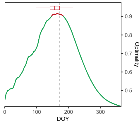
Figure S1: Average optimal trade-off between environmental predictability and growth potential across Europe, with an alternative GDD definition ( T_{lower} = 0^{\circ}\text{C} and T_{upper} = 40^{\circ}\text{C} ).
