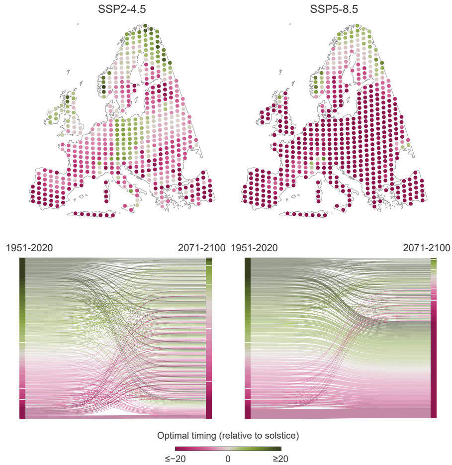
Figure S4: Average optimal timing (??) hides variation in optimal timing across the different future climatic conditions of Europe (2071-2100). On the top panel, sites are sampled on a regular grid across Europe. On the bottom panel, Sankey diagrams show the proportional flow of (site-specific) optimal timing from 1951-2020 to 2071-2100. Colors indicate the timing—relative to the solstice—of the median optimal day.
