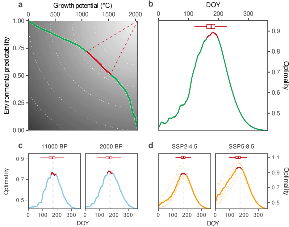
Figure 1: Solstice marks the average optimal trade-off between environmental predictability and growth potential across Europe. (a,b) represent current climatic conditions (1951-2020), (c) represents past climatic conditions (11000 BP and 2000 BP, where BP stand for "Before Present"), and (d) represents future climatic conditions (2070-2100, for two emission scenarios, SSP2-4.5 and SSP5-8.5). In (a), environmental predictability measures how well GDD by a given day predicts total yearly GDD ( R^2 of a linear regression across years), while growth potential represents the remaining GDD from that day onward. In (b,c,d), optimality is based on the Euclidean distance from the (unattainable) perfect point where both predictability and growth potential are maximized (illustrated by the red dashed lines and the gray gradient in (a)). The red sections of the curves represent days where optimality falls within the 90th percentile (i.e. top 10% most optimal days). GDD range was defined between 5°C and 35°C. Note that we did not consider moisture availability constraints along the growing season, that will likely increase with climate change (Garonna et al., 2018; Zhao and Running, 2010; Seo et al., 2025).
