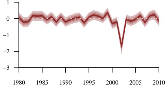
Residuals - tree 10
