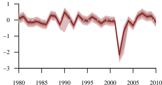
Residuals - tree 7
