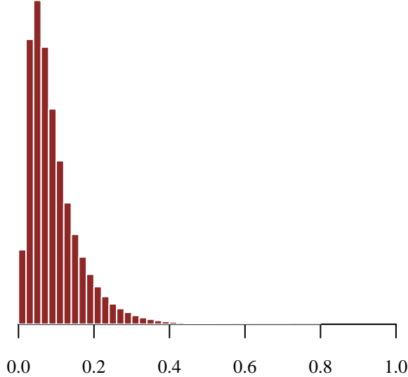
\text{inv\_logit}(\mu_{\alpha\_sck})
