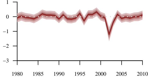
Residuals - tree 21
