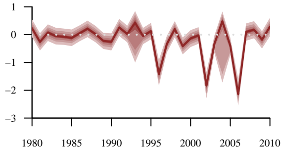
Residuals - tree 17
