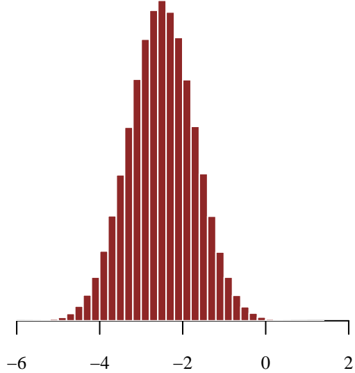
\mu_{\alpha\_sck}
