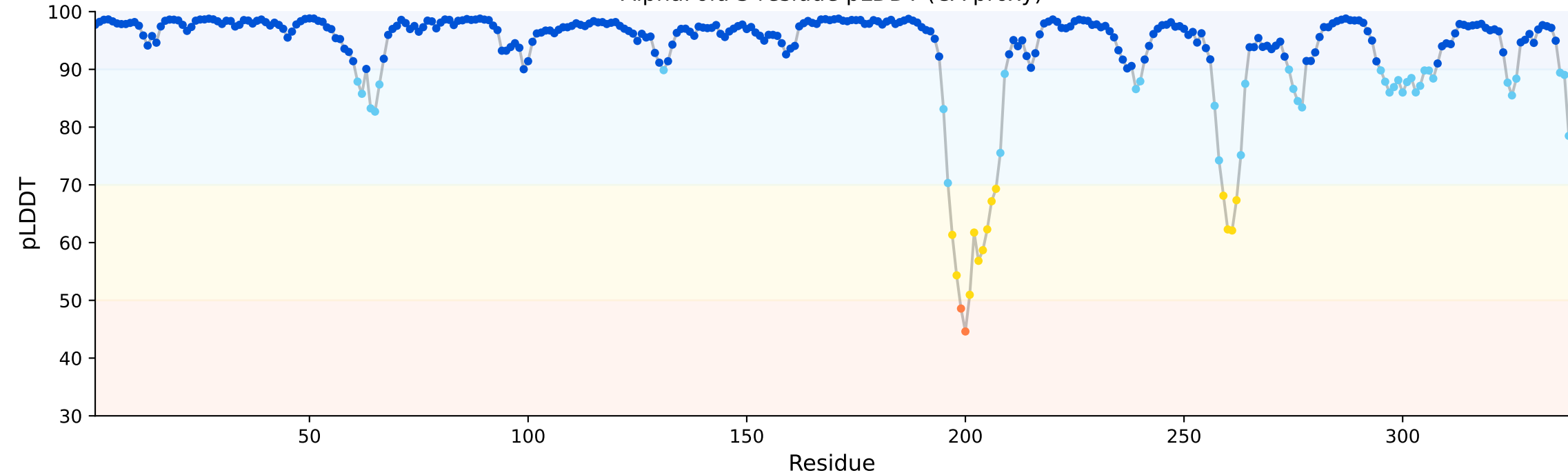
AlphaFold 3 residue pLDDT (CA proxy)
