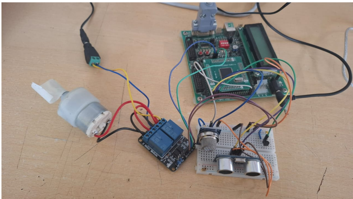
Figure 2: Hardware implementation of the motor safety interlock system on LPC1768
