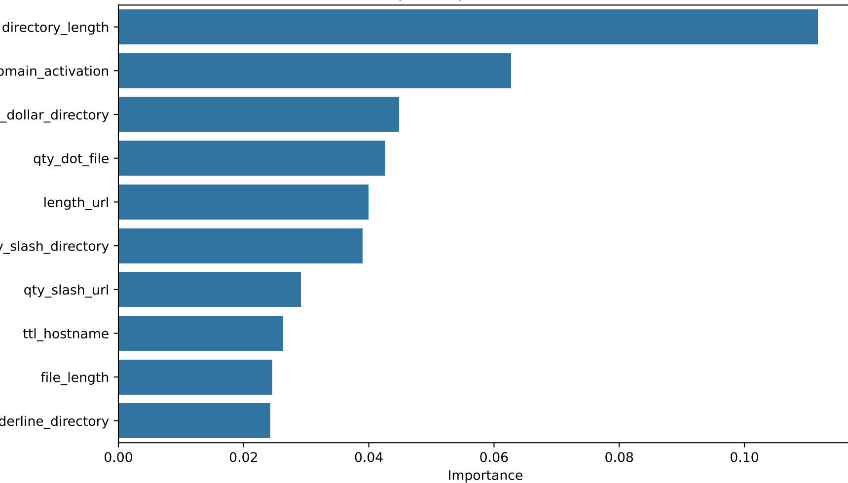
Top 10 Important Features
