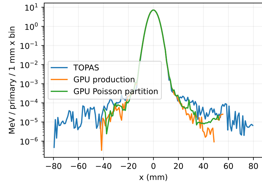
z = 18.00 mm; 2 mm slab
