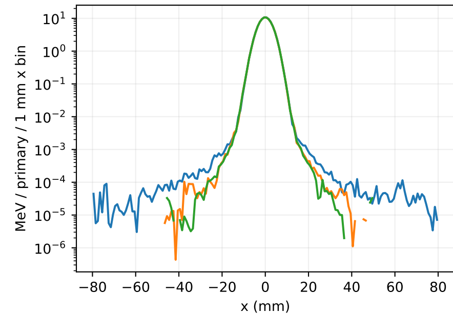
z = 27.00 mm; 2 mm slab
