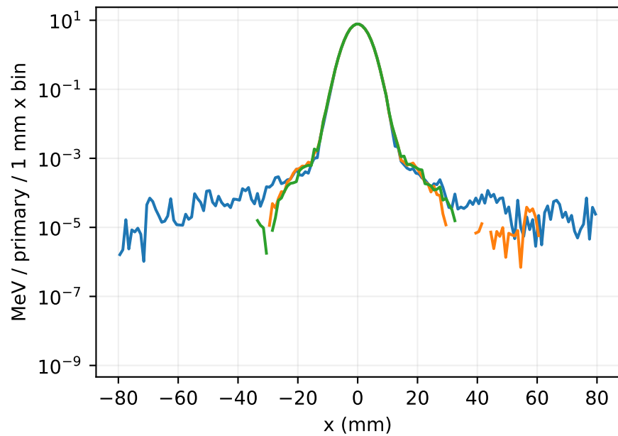
z = 23.00 mm; 2 mm slab
