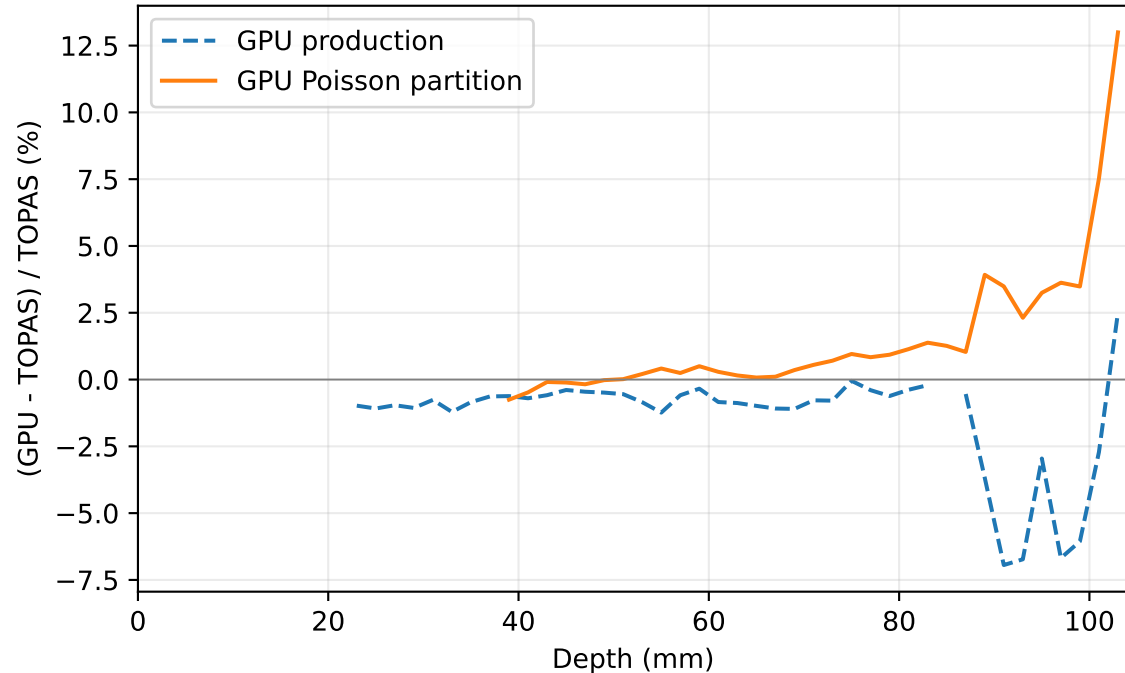
b1_200 core relative error
