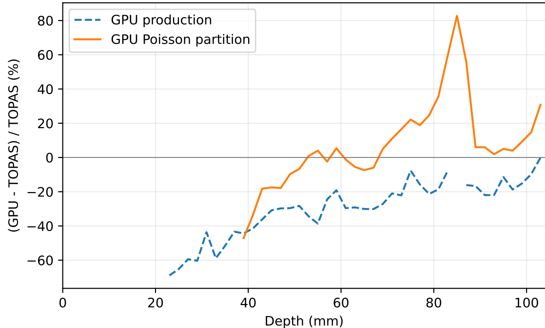
b1_200 halo relative error
