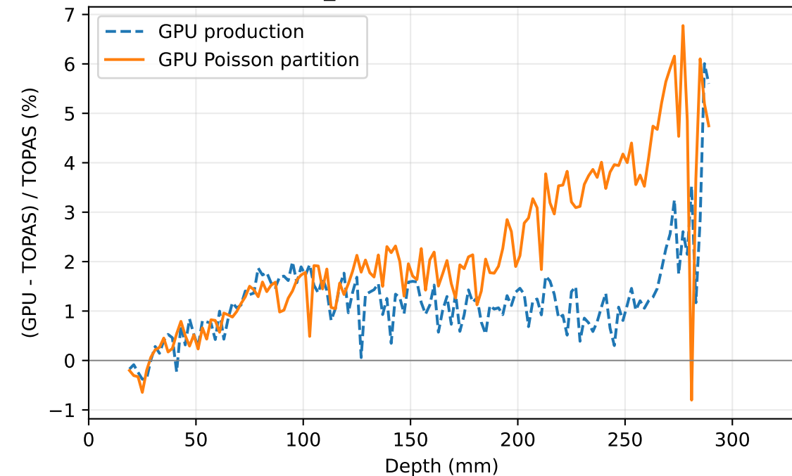
b1_400 core relative error
