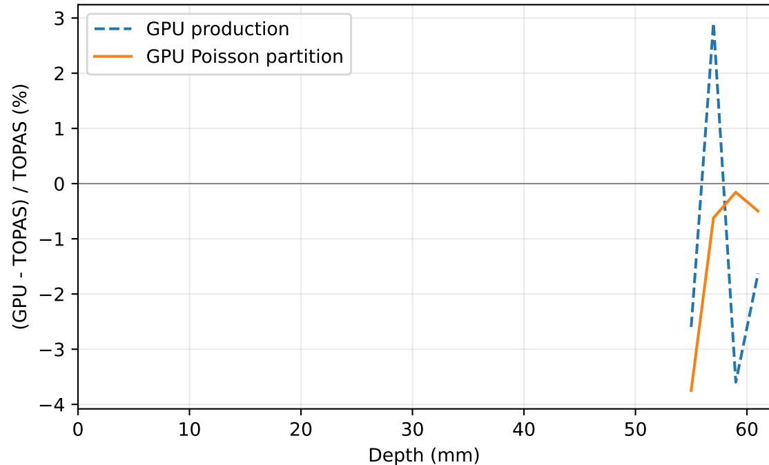
b2_150 core relative error
