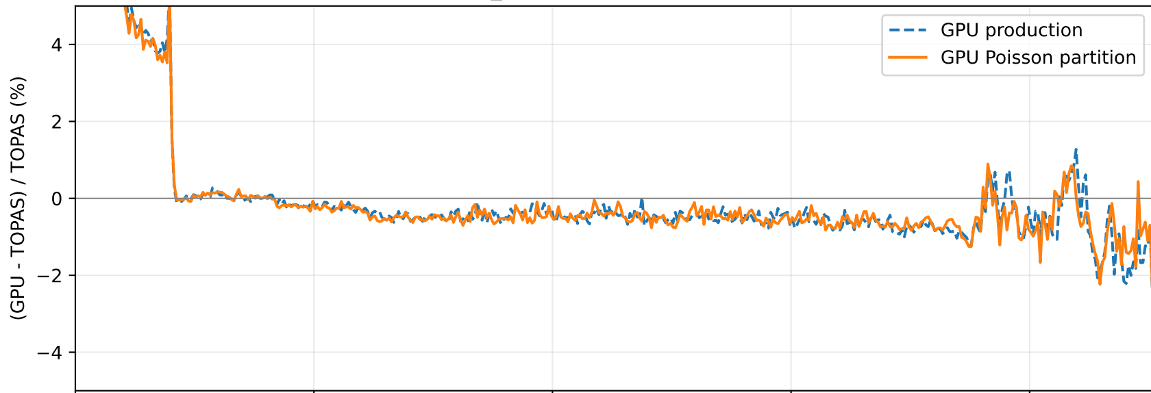
b3_layers IDD relative error
