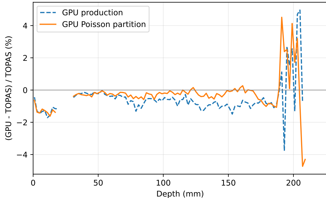
b3_layers core relative error
