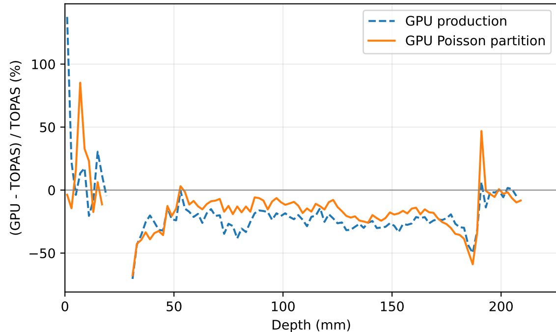
b3_layers halo relative error
