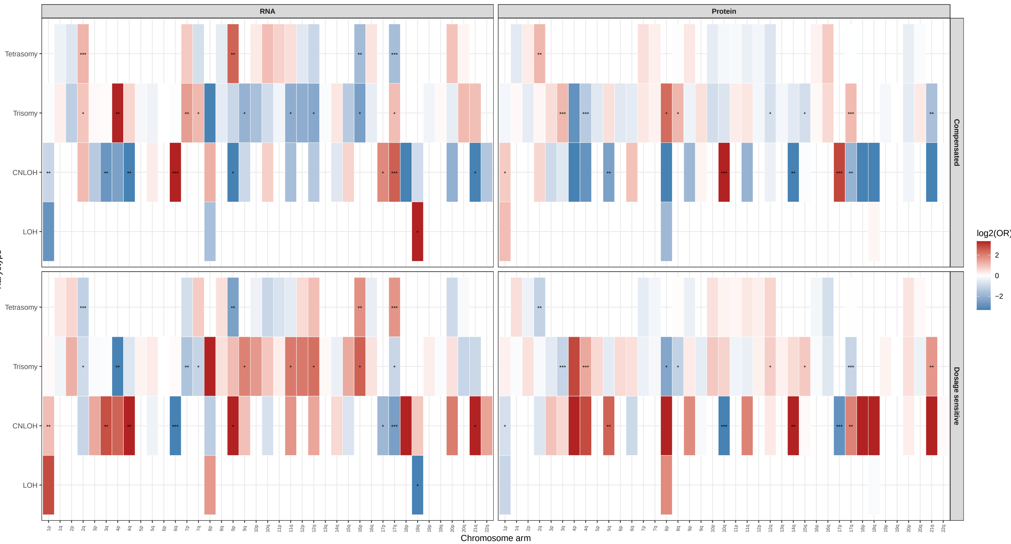
Per-arm enrichment: compensated vs dosage sensitive
