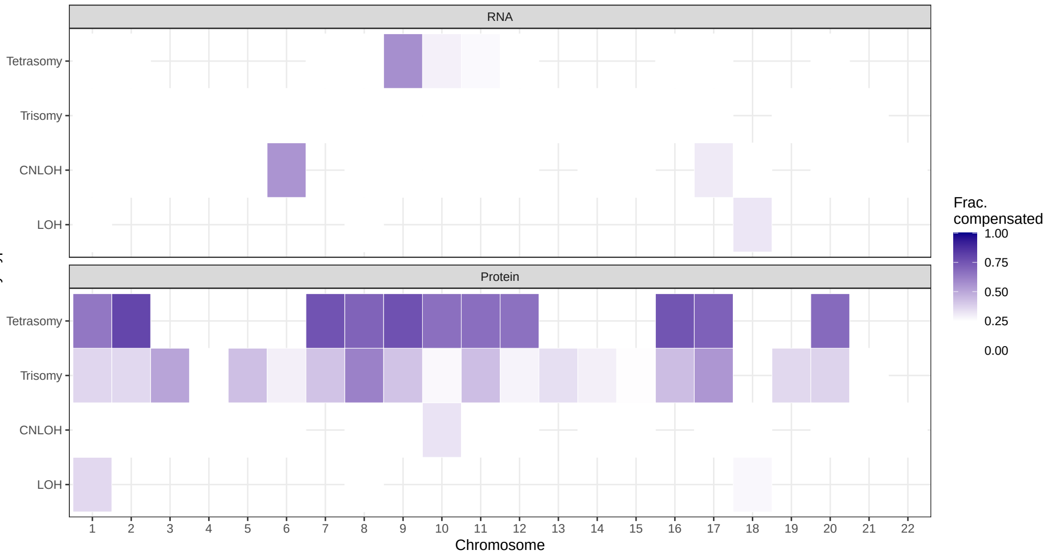
Raw fraction compensated per chromosome
