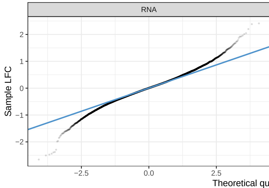
Q-Q vs Gaussian fit (blue). S-shape = heavy tails
