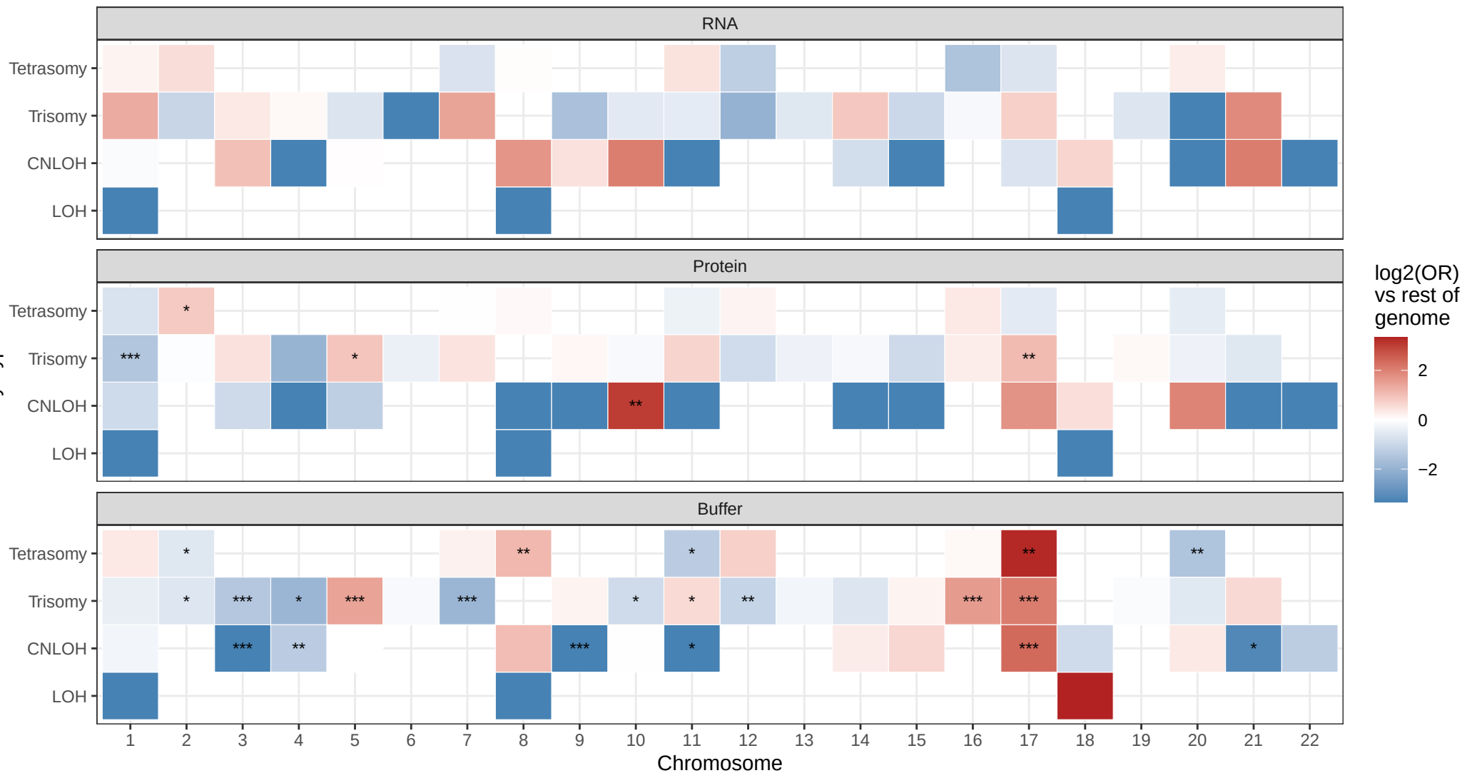
Fisher enrichment per chromosome (stars = BH-adjusted p)
