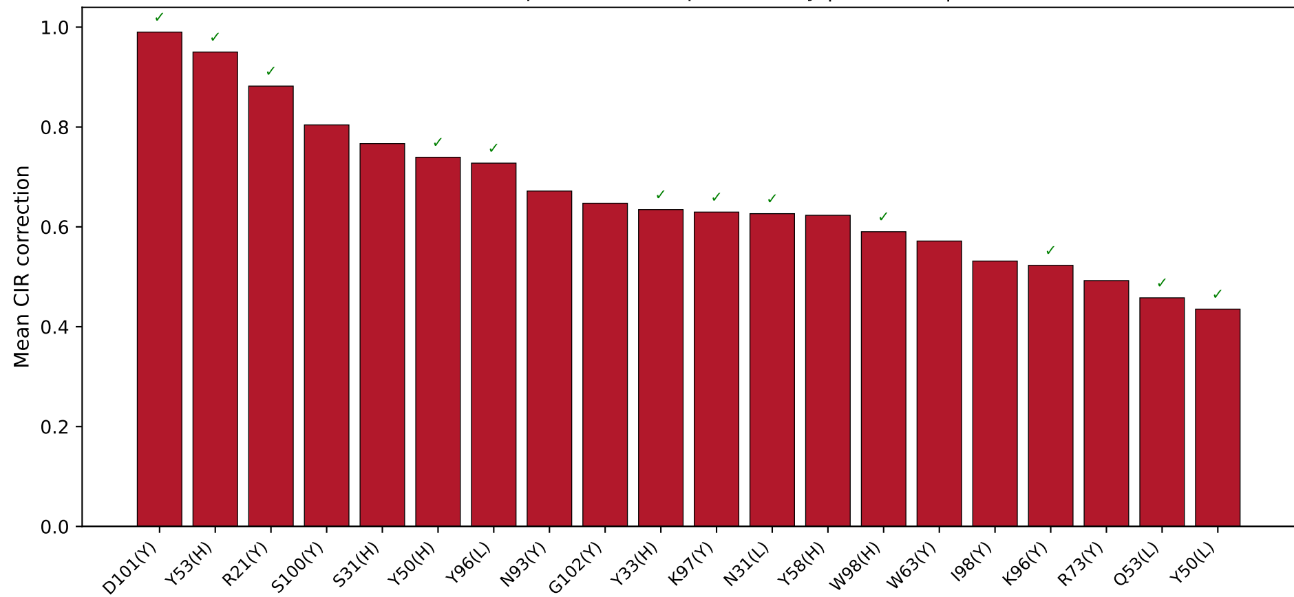
3HFM: Top 20 interface positions by |correction|
