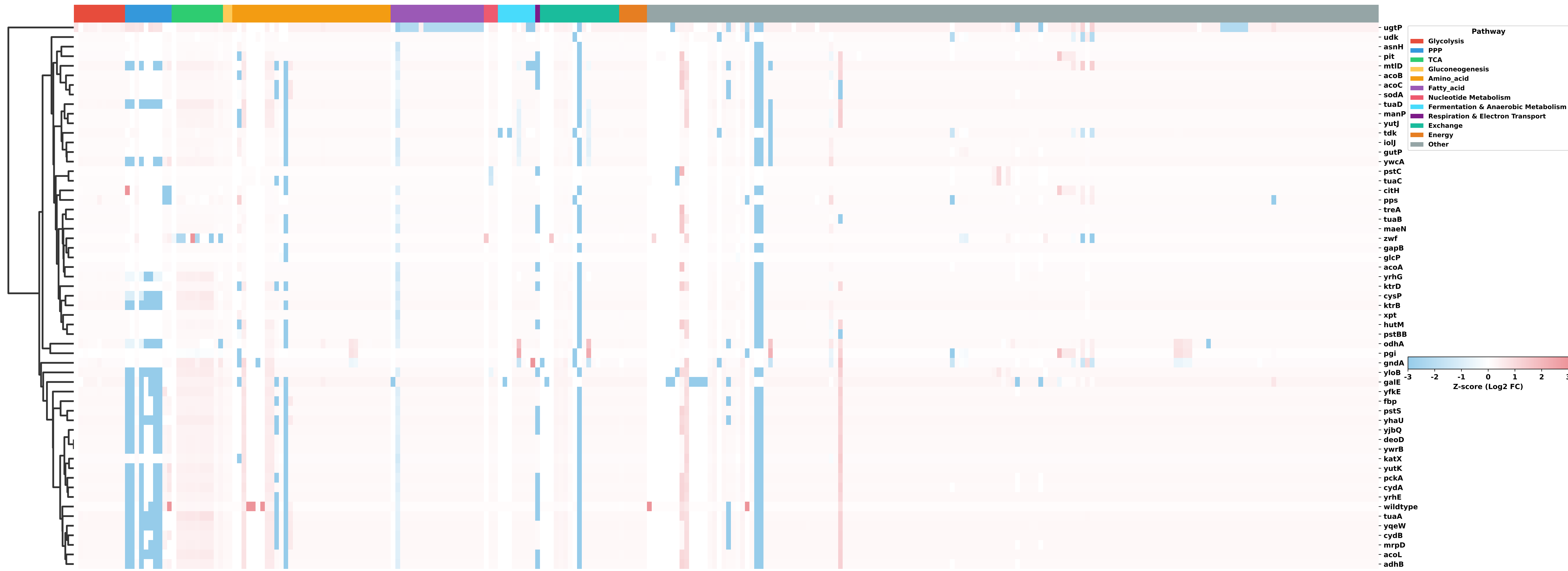
fba - Clustered Heatmap (Row Z-score normalized)
