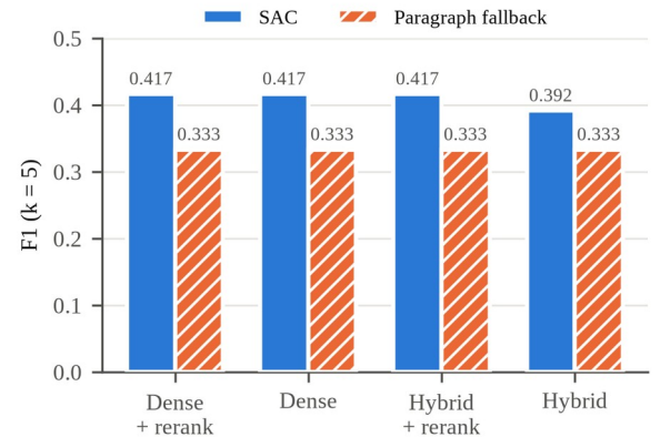
Fig. 4. Retrieval F1 for SAC and paragraph chunking under each retrieval setting.
