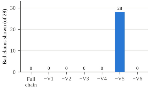
Fig. 5. Corrupted claims shown to the user when each layer is removed (28 in total). Only removing the V5 gate lets them through.
