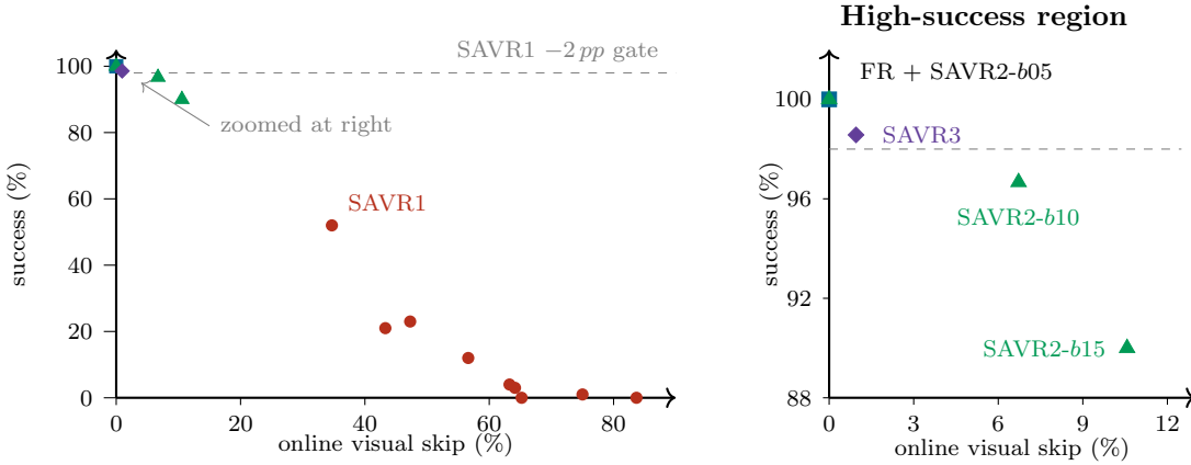
Figure 2: Observed success-efficiency frontier with the crowded high-success region expanded at right. The coincident FR and zero-reuse SAVR2-b05 results share one coordinate. SAVR1 used 100 episodes per point, SAVR2 used 30 per point, and SAVR3 used 70; the plot is descriptive because the staged populations differ.
