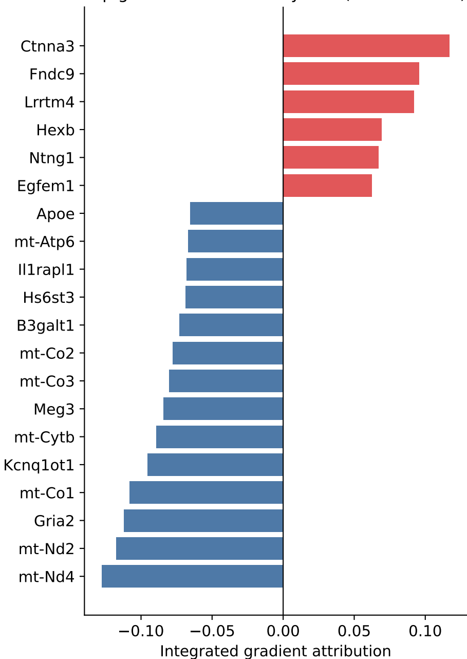
Top genes: shared-toxicity axis (IG attribution)
