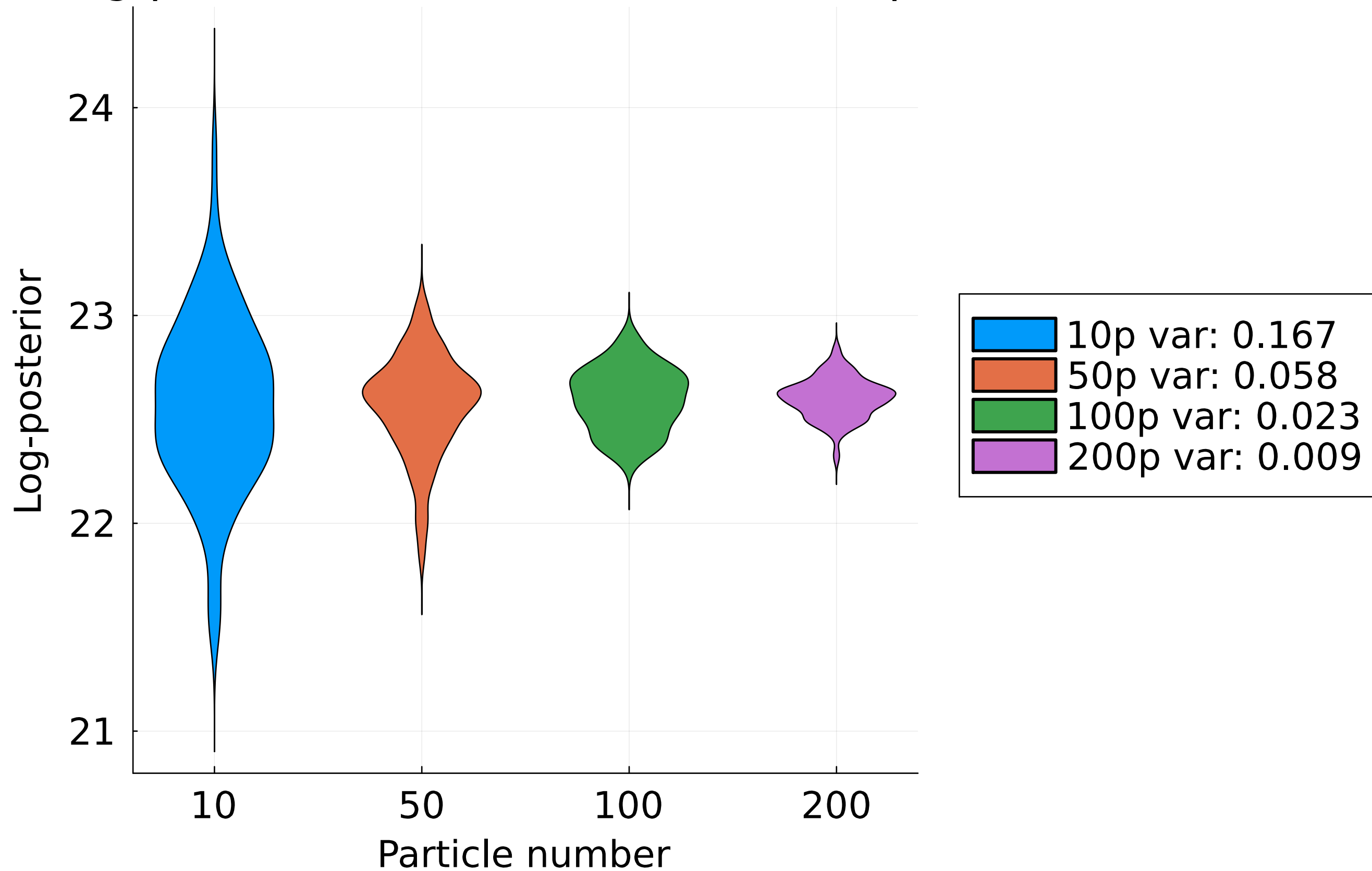
el: log-posterior estimates for different particle numbers
